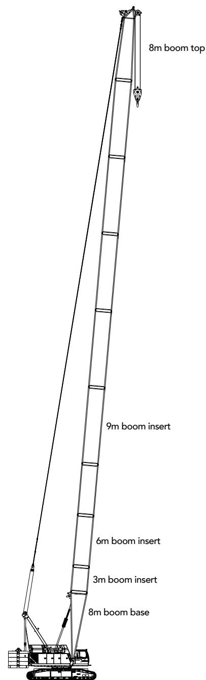
H Configuration (16m~76m)
