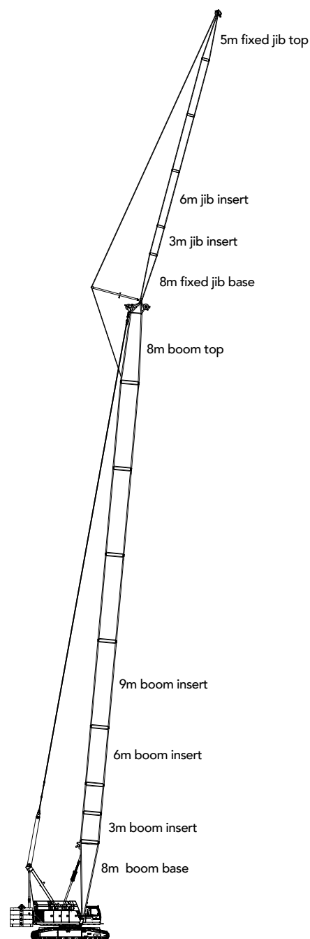
FJ Configuration (28~64m)+(13~31m)
