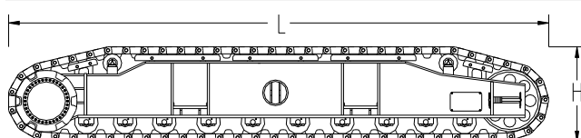
Track carrier assy.
