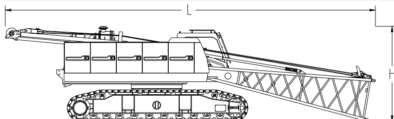
Basic machine 1 (with pivot section and tracks on)
