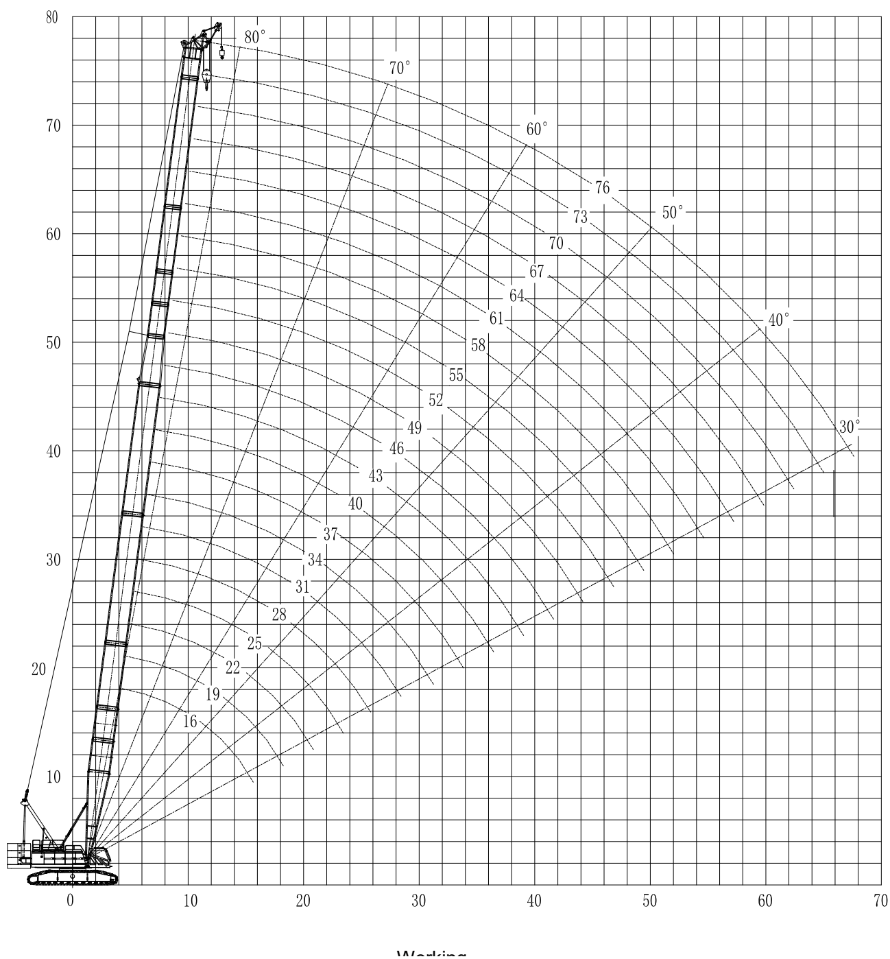
Hoisting height curves (S)
