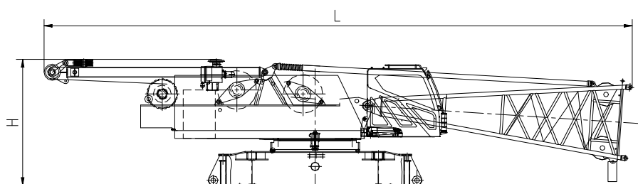
Basic machine 1
